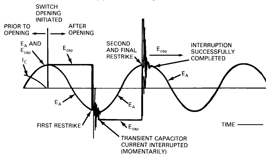
(b) Transient overvoltage character due to switch restrike during interruption
